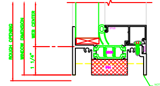
201 SILL 325 FIXED | CASEMENT IN
