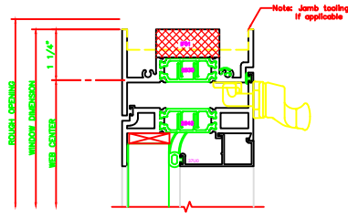
110 HEAD 325 PROJECT IN OW LOCK
